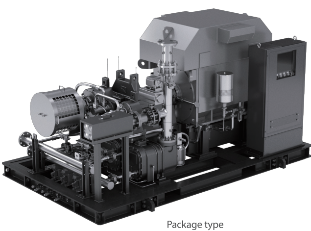
Package type
